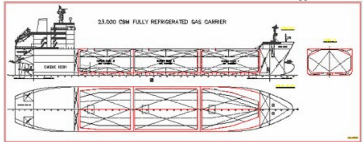
Gas carrier 23.000 m 3 with dehonit® / Permalı Tank Supports
