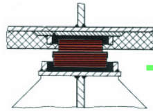
Moveable bearing
