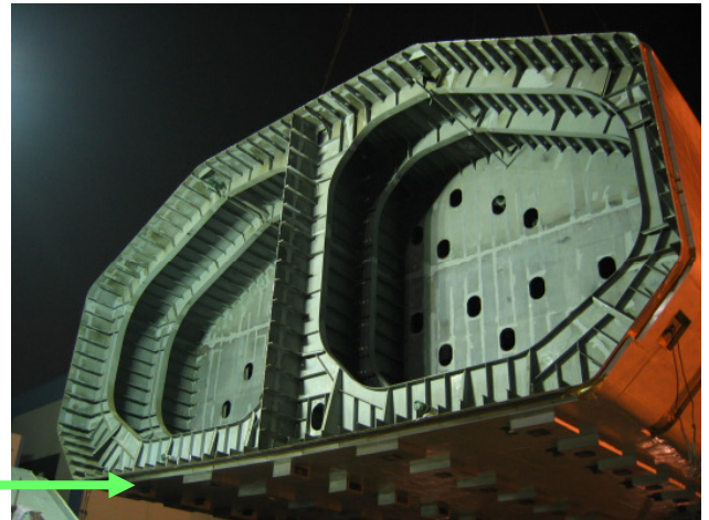
Gas carrier 23.000 m 3 with dehonit® / Permalı Tank Supports
